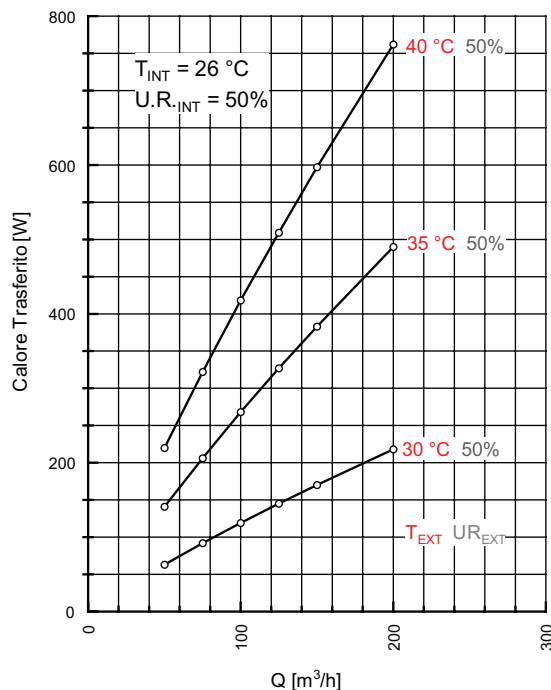
Raffrescamento ( T_{int} = 26^{\circ}; 30^{\circ} < T_{ext} < 40^{\circ} )
